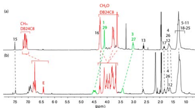
Figure 3. ^1\text{H} NMR spectra (400 MHz, \text{CD}_3\text{CN} , 298 K) of (a) the uncomplexed compound 7u and (b) the lasso rotamacrocycle 7 . The coloring, lettering and numbering correspond to the proton assignments indicated in Scheme 1.
