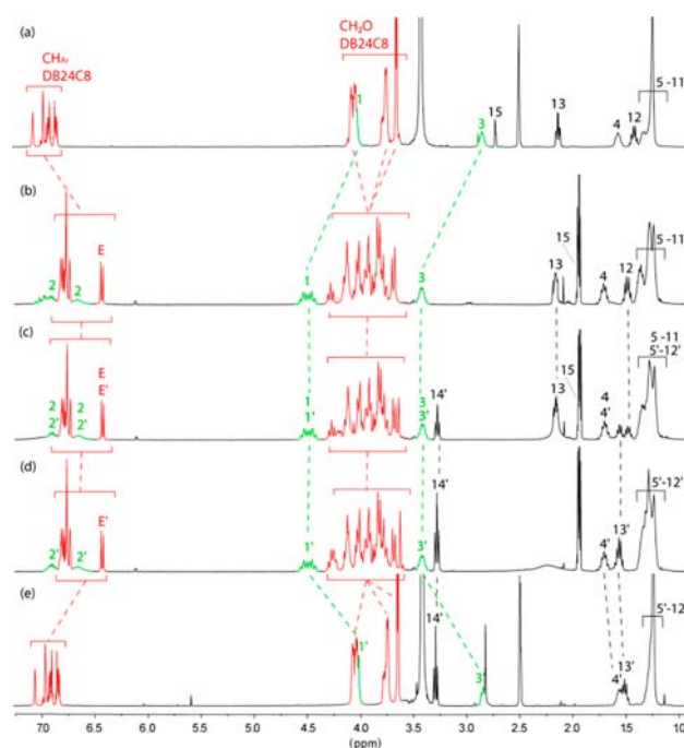
Figure 1. 1 H NMR spectra (400 MHz, 298 K) of (a) the uncomplexed alkyne compound 5u in DMSO- d 6 , (b) the dialkyne pseudo rotaxane dimer 5 in CD 3 CN, (c) the stoichiometric mixture of pseudorotaxane dimers 3 and 5 in CD 3 CN, (d) the diazido pseudo rotaxane dimer 3 in CD 3 CN, and (e) the uncomplexed azido compound 3 in DMSO- d 6 . The coloring, lettering, and numbering correspond to the proton assignments indicated in Scheme 1.
