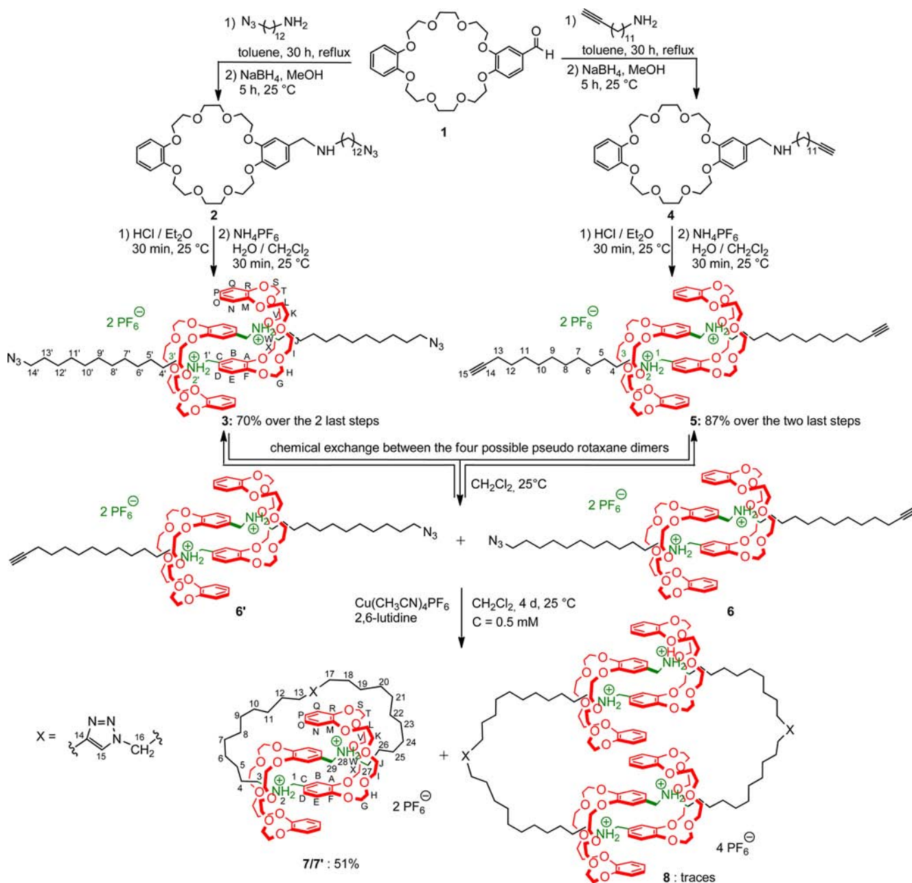
Scheme 1. Synthesis of the Two Symmetrical Diazide and Dialkyne [c2]Daisy Chains 3 and 5 , Equilibrium between Pseudorotaxanes 3 , 5 , and 6/6' , and Synthesis of the Double-Lasso Rotamacrocycle Enantiomers 7/7'
