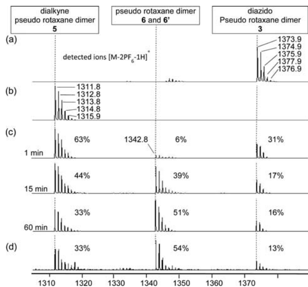
Figure 2. MALDI-TOF mass spectra of (a) the diazido pseudorotaxane dimer 3 , (b) the dialkyne pseudorotaxane dimer 5 , (c) a stoichiometric mixture of pseudorotaxane dimers 3 and 5 over time, and (d) after protonation of a stoichiometric mixture of monomers 2 and 4 .
